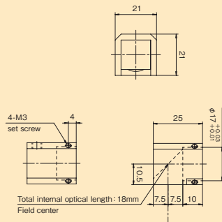
MPM-2 For \phi 17 lens tube Total internal optical length 18mm
