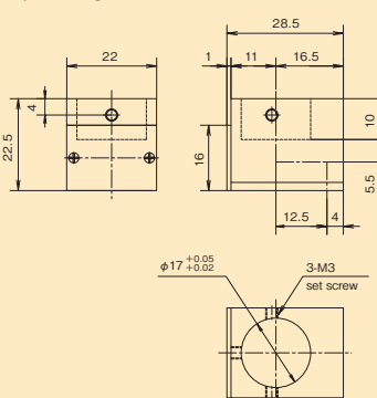
MPM-5 For \phi 17 lens tube Total internal optical length 26mm
