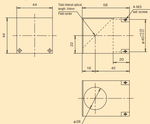
PM-2- \phi 40 For \phi 40 lens tube Total internal optical length 44mm
