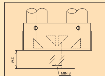
Dual right angle prism mount
