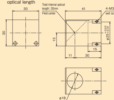
PM-2- \phi 25 For \phi 25 lens tube Total internal optical length 30mm
