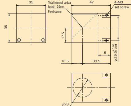
PM-2- \phi 29.5 For \phi 29.5 lens tube Total internal optical length 36mm
